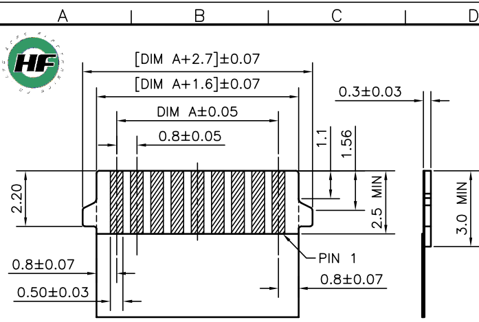
RECOMMENDED FPC/FFC DIMENSIONS GENERAL TOLERANCE ±0.05
